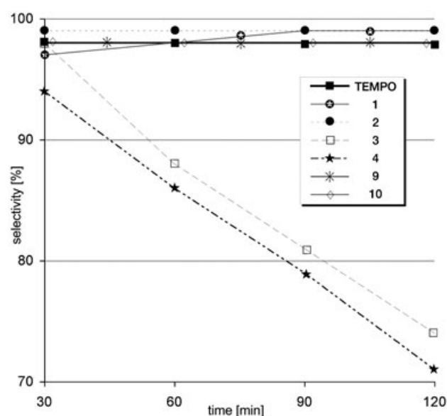
Figure 3. Oxidation of 1-octanol to octanal with BAIB. Selectivity profiles for reactions mediated by fluorine-tagged TEMPO radicals.
