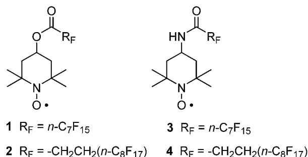
Figure 1. Light fluorous TEMPO radicals.
