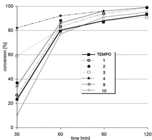
Figure 2. Oxidation of 1-octanol to octanal with BAIB. Conversion profiles for reactions mediated by fluorine-tagged TEMPO radicals.
